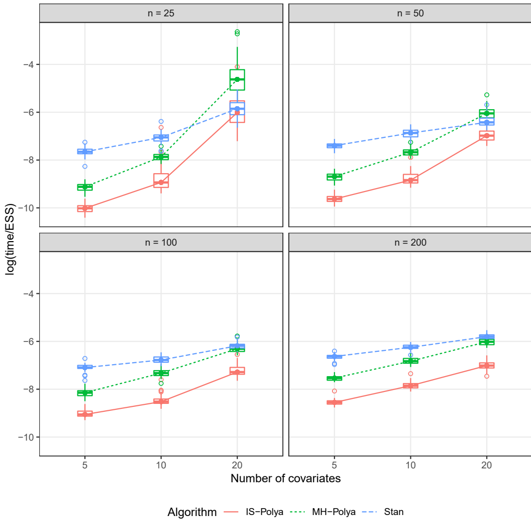
FIGURE 2.1: Time per independent sample (in logarithmic scale) for the three algorithms. For each combination of n and p the boxplots represent the distribution of the (log) time (in seconds) over the effective sample size using a Gaussian prior, over 50 replications.
